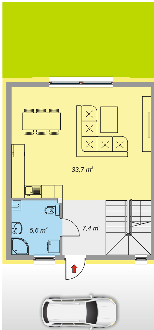
PARTER
